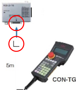
CON-TG用TPアダプタ RCB-LB-TG
