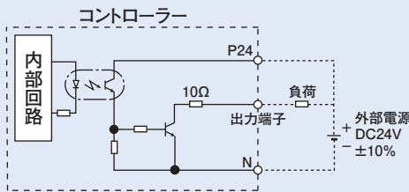
NPN仕様
