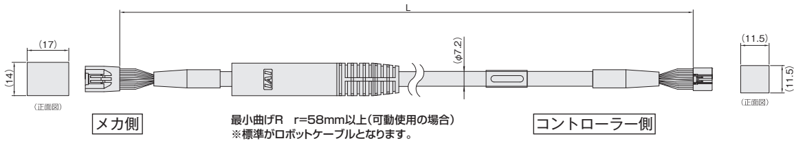
DF62B-13EP-2.2C(18)
