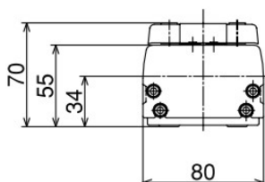
RCS-SM-150
